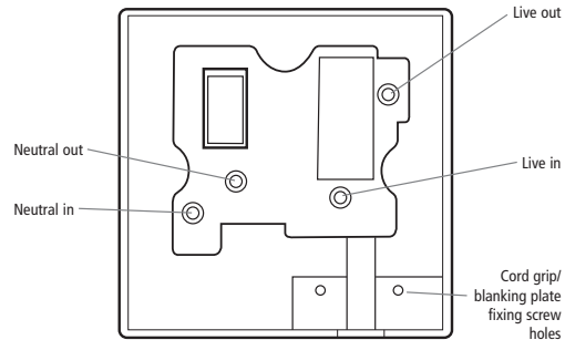
Fig. 2 TGBT4 Rear Connections
