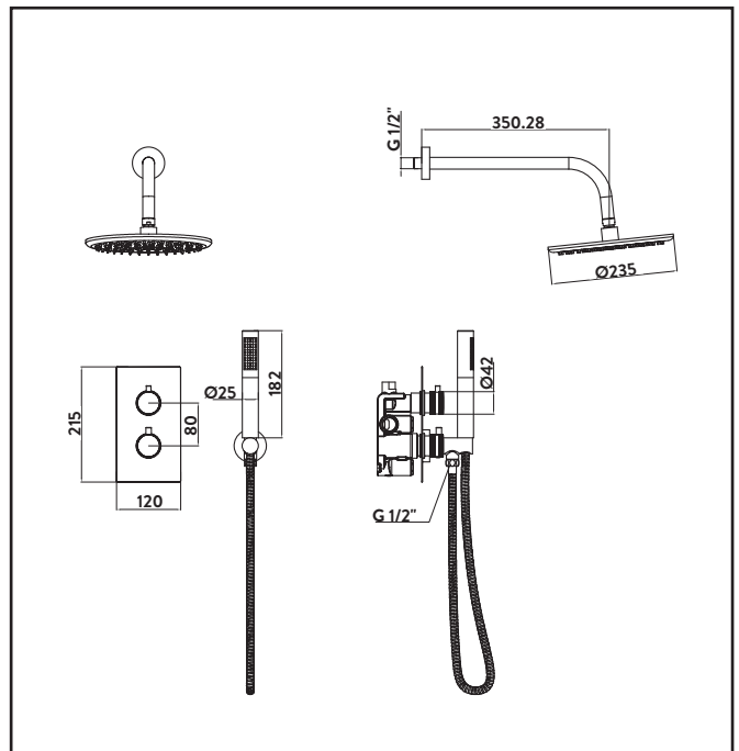
Dimensions (measurements in mm)
